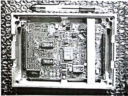
Fig. 7. Electronic board employed to validate the uploading software.
